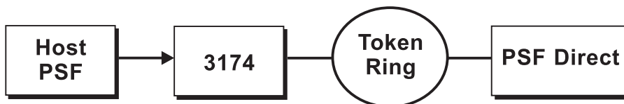
Figure 5. Local 3174 Configuration: Simplified View
