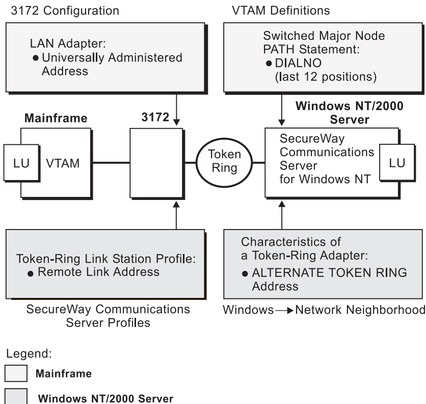
Figure 15. Network Addresses for Local 3172 Configuration
