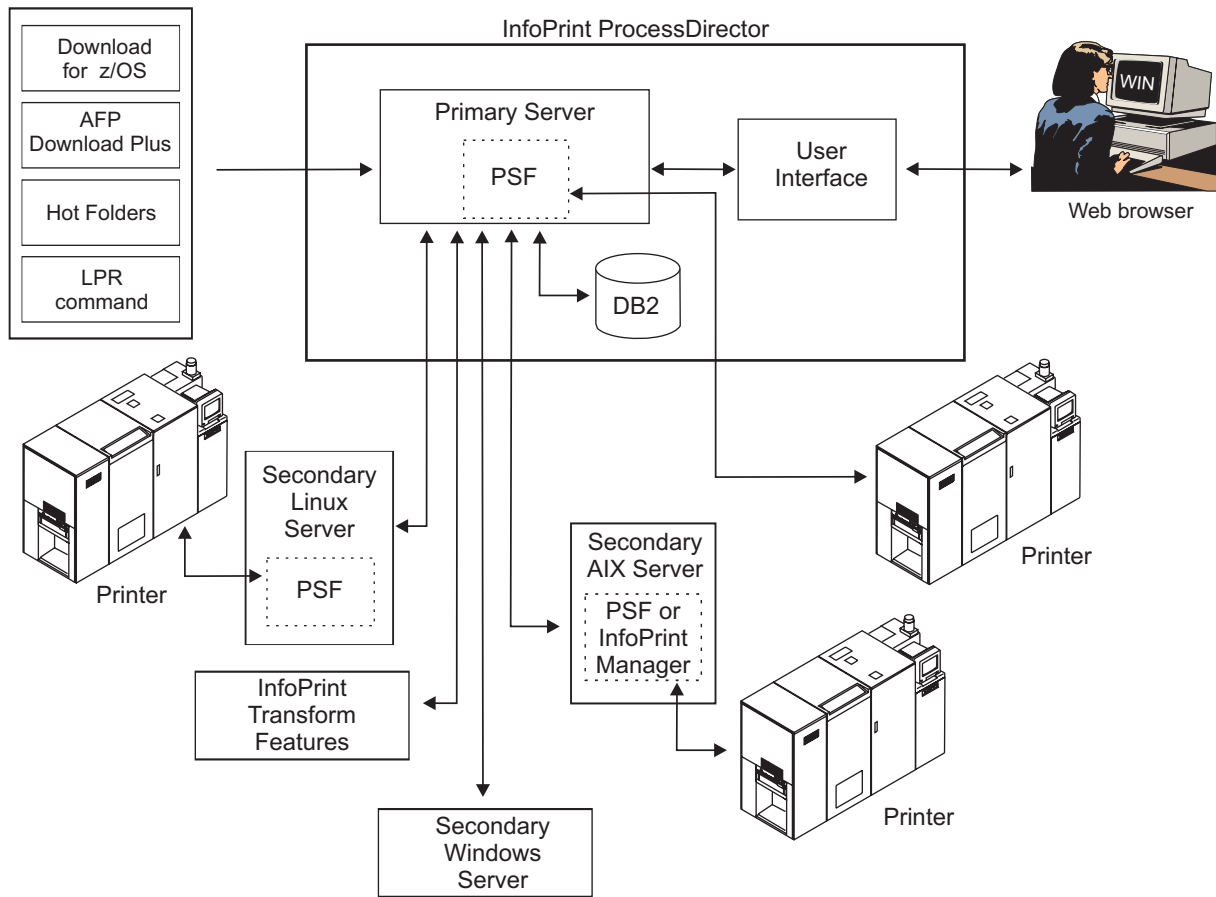
Figure 1. Example of an InfoPrint ProcessDirector system configuration
