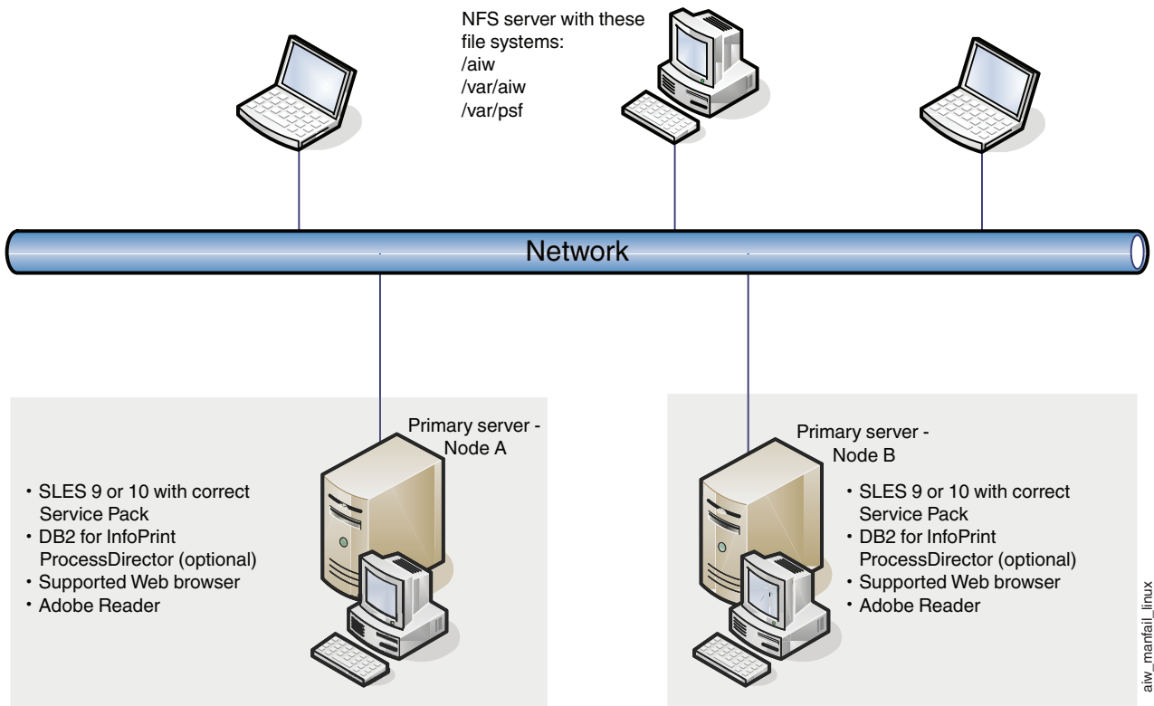
Figure 2. Example of a configuration with active and backup primary servers using an NFS server
