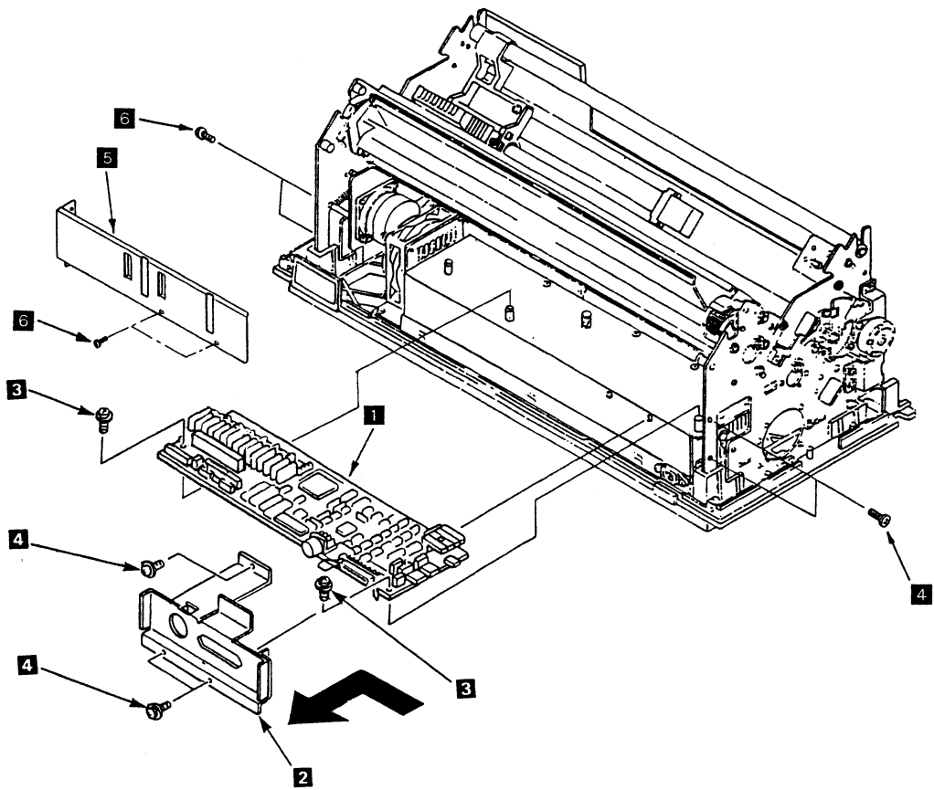
図 6-5. Logic Card
