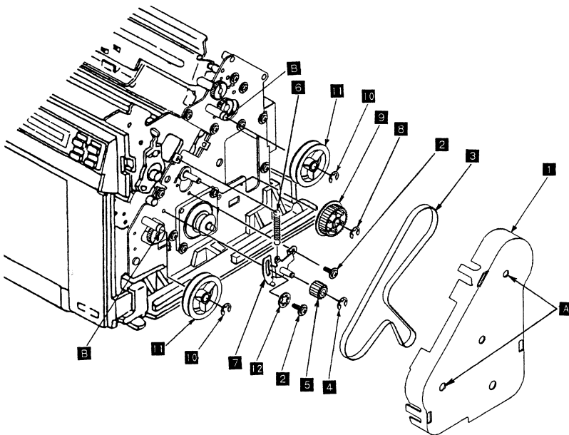
図 6-17. Feed Belt, Pulleys, Gears
