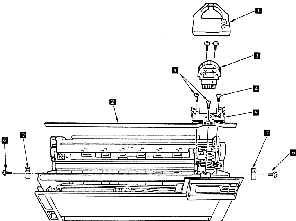
図 6-10. Ribbon Drive Assembly
