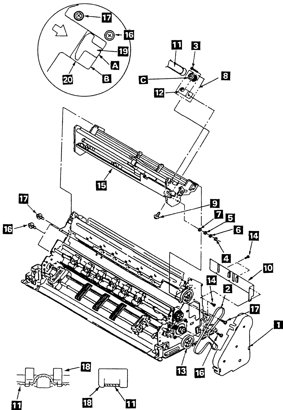
図 6-13. Tension Pulley Assembly
