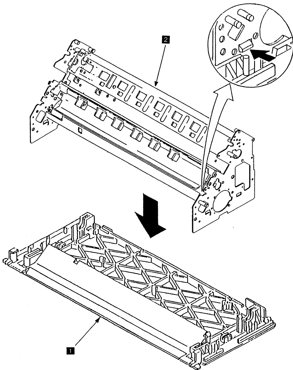
図 6-31. Feed Frame Assembly
