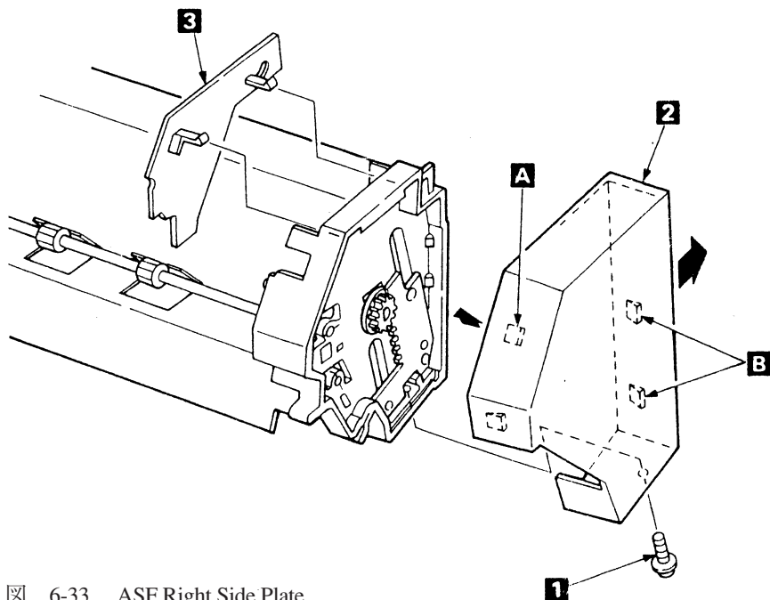
図 6-33. ASF Right Side Plate
