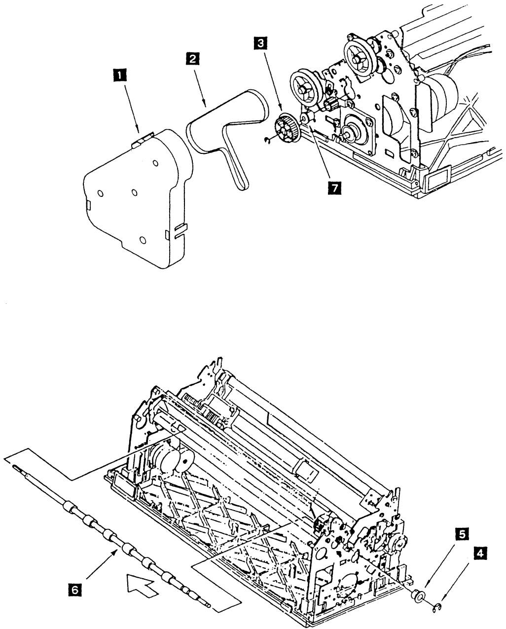
図 6-23. Lower Feed Roller Shaft, Bushing
