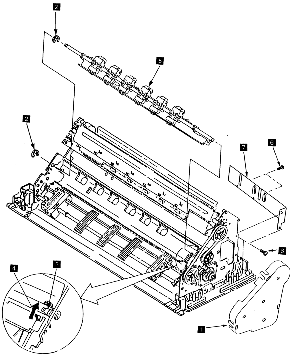
図 6-24. Lower Pressure Rollar Assembly
