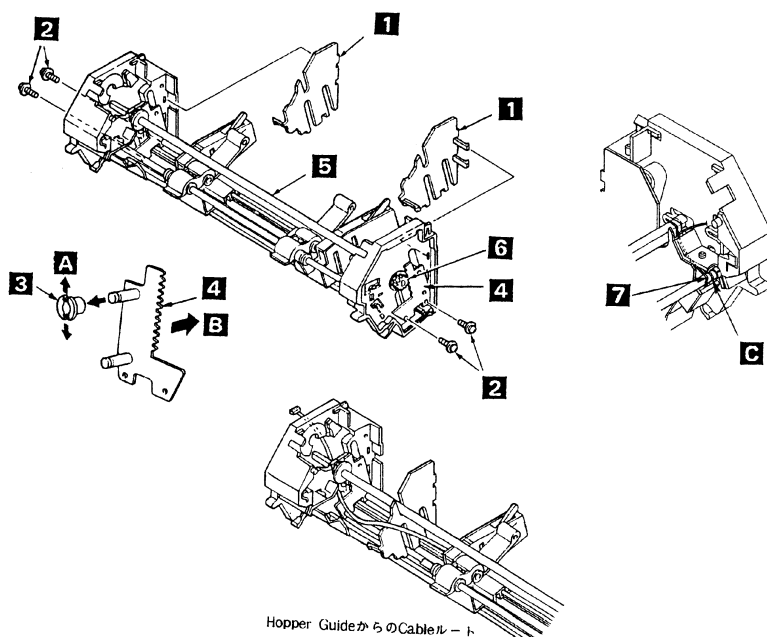
図 6-41. ASF Lift Shaft/Slider
