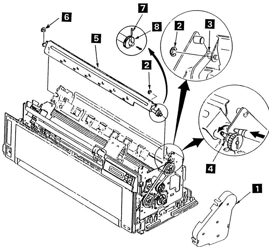
図 6-20. Upper Pressure Roller Assembly, Gear
