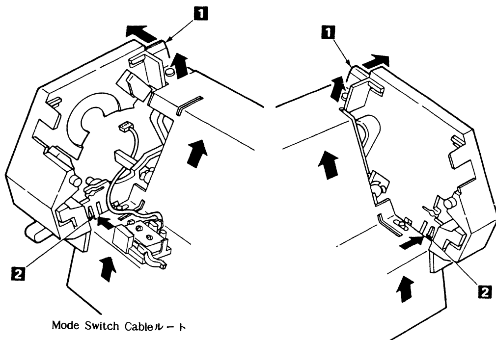
図 6-39. ASF Support Guide
