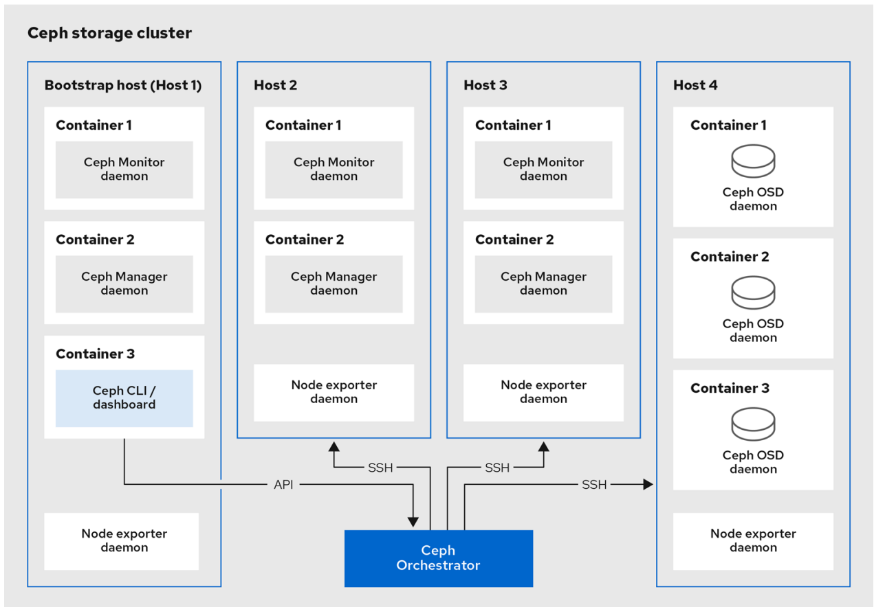
Figure 1. Ceph storage cluster deployment
