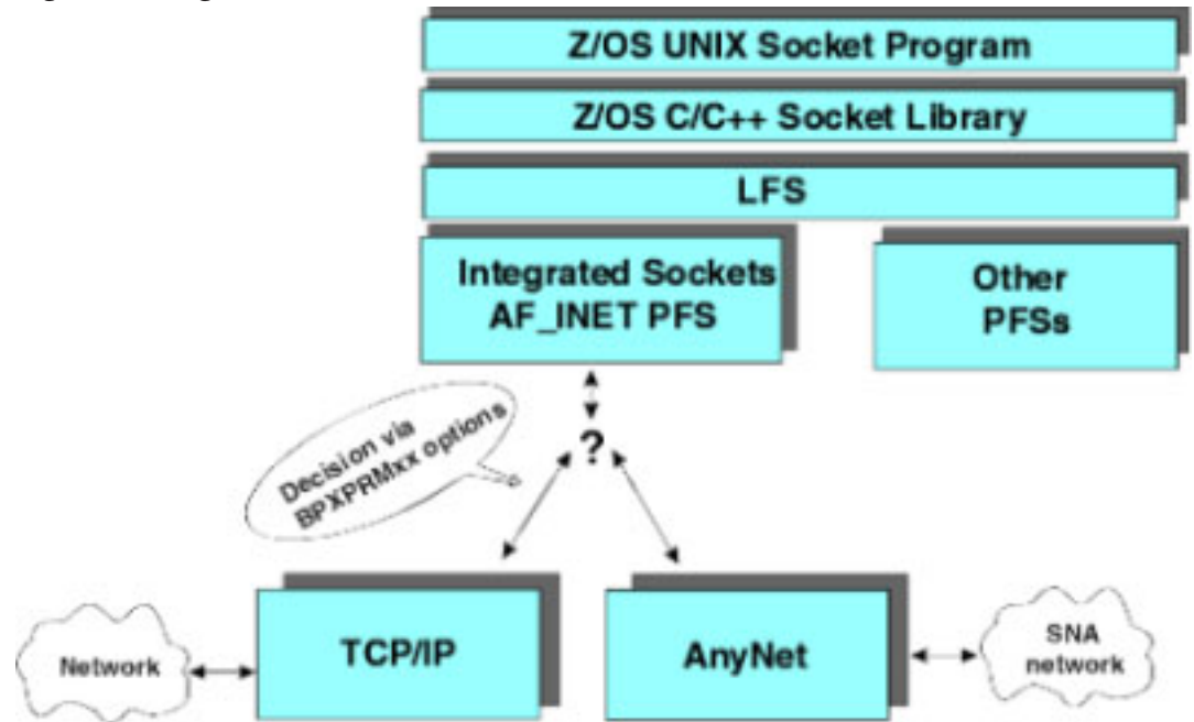
Figure 2. Integrated sockets
