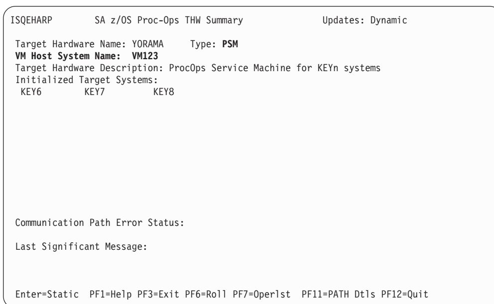
Figure 30. Processor Operations Target Hardware Summary Panel (ISQEHARP) for PSMs
