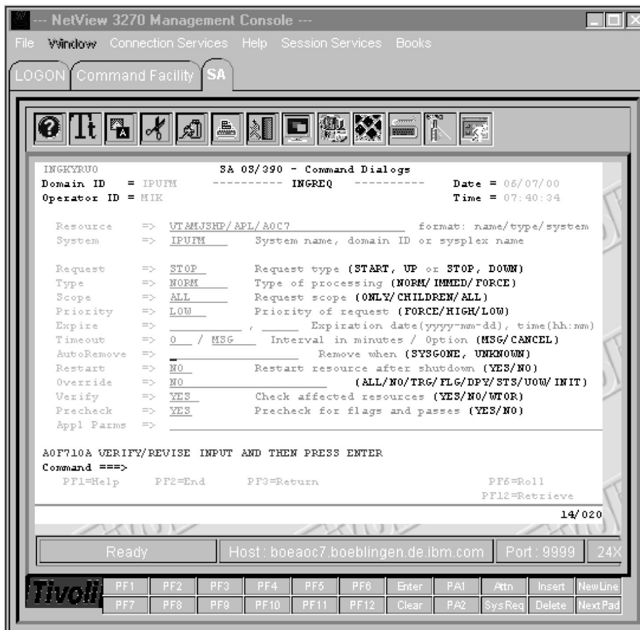
Figure 61. NetView Console with INGREQ Panel
