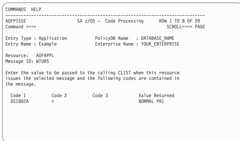
Figure 14. Code Processing Panel for an Application Resource
