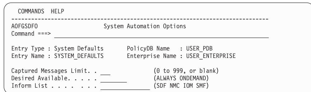
Figure 217. System Automation Options Panel
