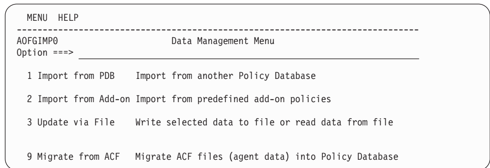
Figure 260. Data Management Menu Panel
