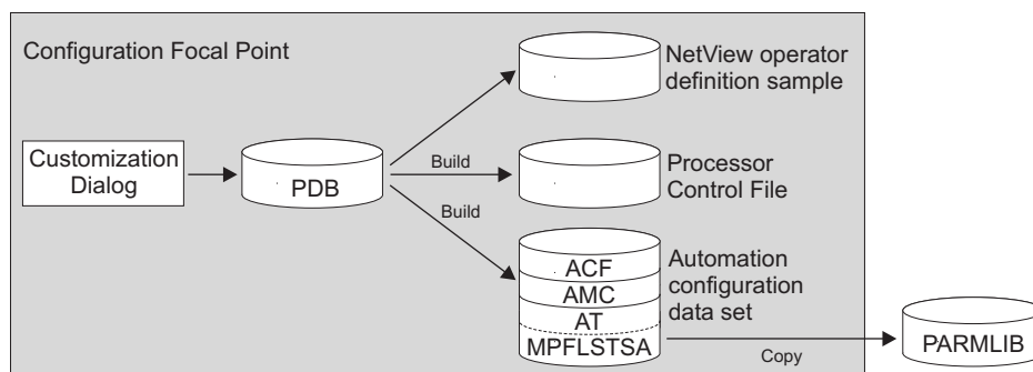
Figure 256. Configuration File Build
