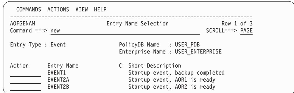
Figure 158. Entry Name Selection Panel for Events
