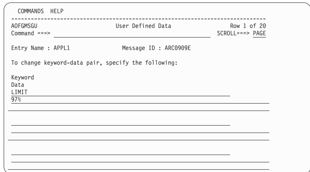
Figure 120. User Defined Data Panel
