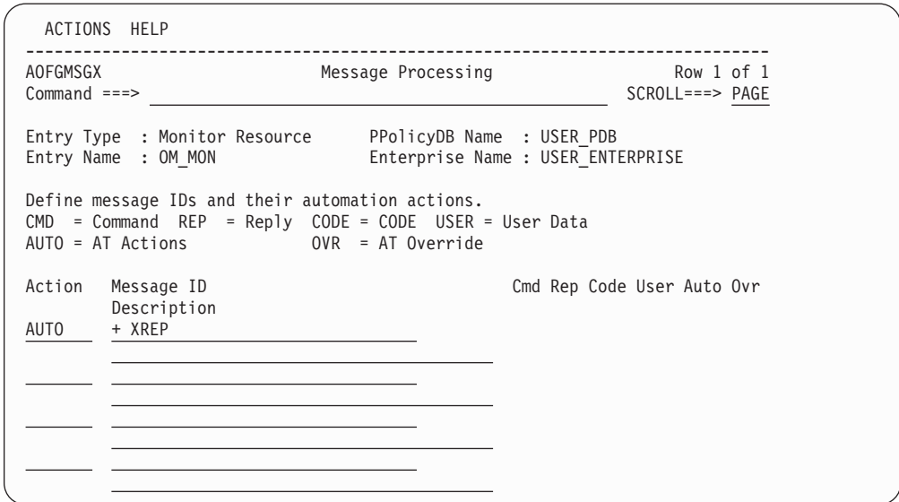
Figure 176. Message Processing Panel with OMEGAMON Exception
