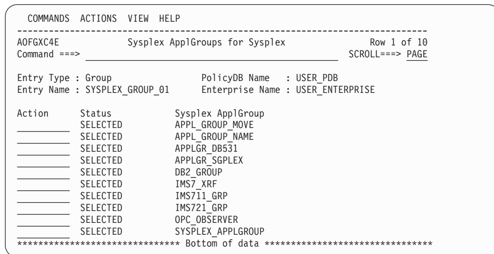
Figure 76. Group Information Panel for Standard Groups
