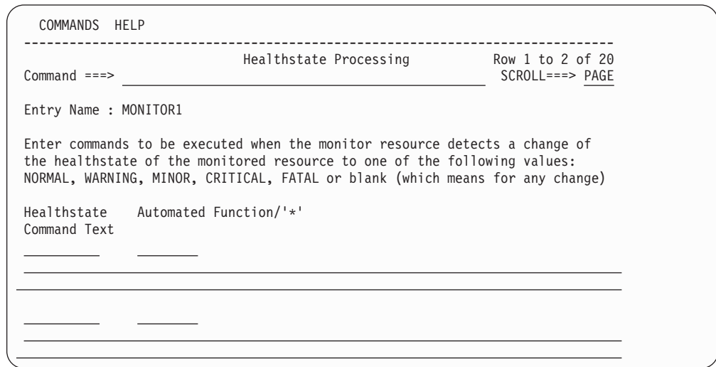
Figure 183. Healthstate Processing Panel
