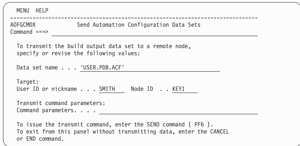
Figure 286. Send Automation Configuration Data Sets Panel
