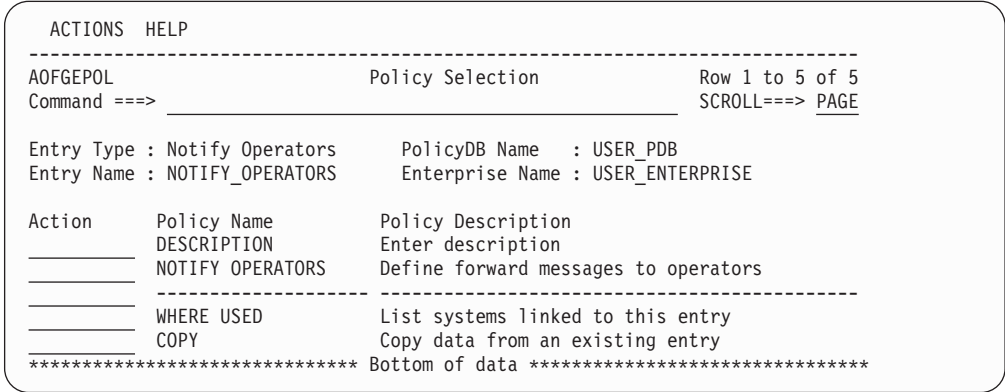
Figure 222. Policy Selection Panel for Notify Operators
