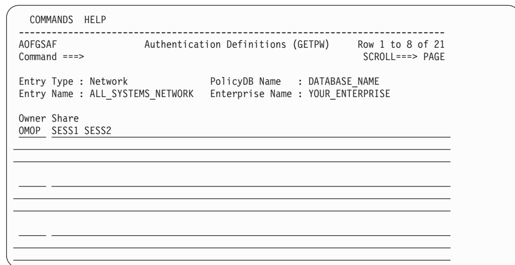
Figure 231. Authentication Definitions Panel
