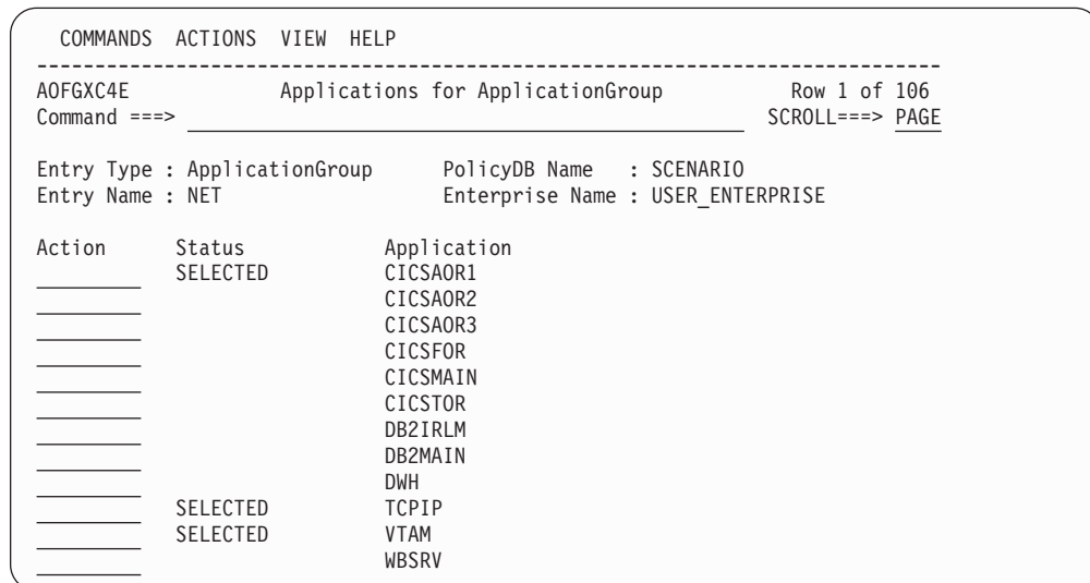
Figure 98. Applications for ApplicationGroup Panel for System Application Groups
