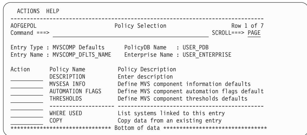
Figure 215. Policy Selection Panel for MVSCOMP Defaults
