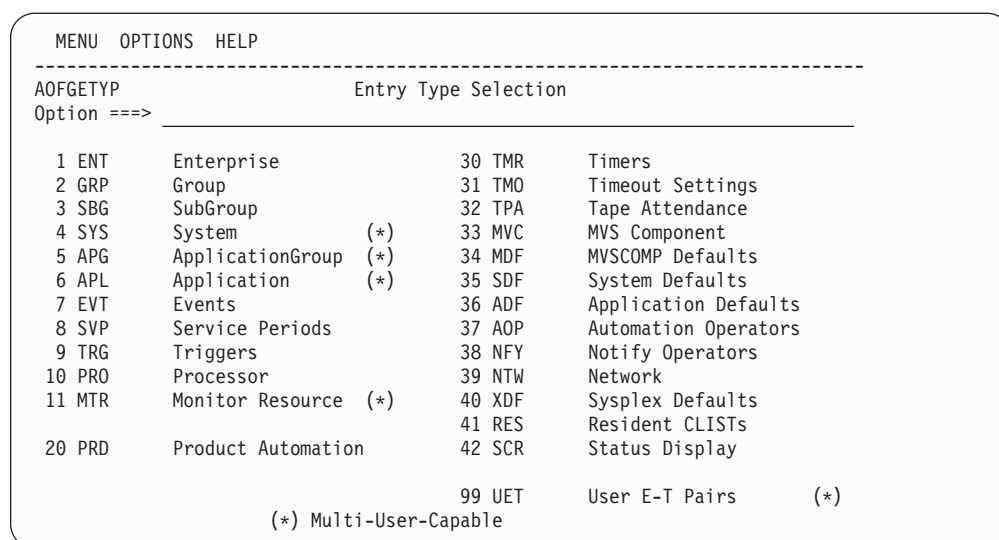
Figure 2. Entry Type Selection Panel
