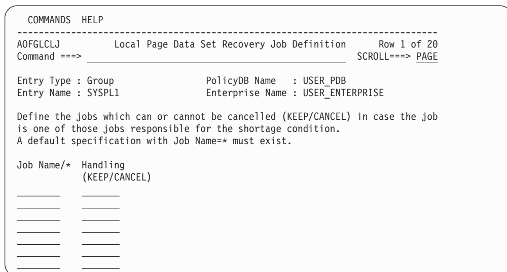
Figure 78. Job Definitions for Local Page Data Set Recovery Panel
