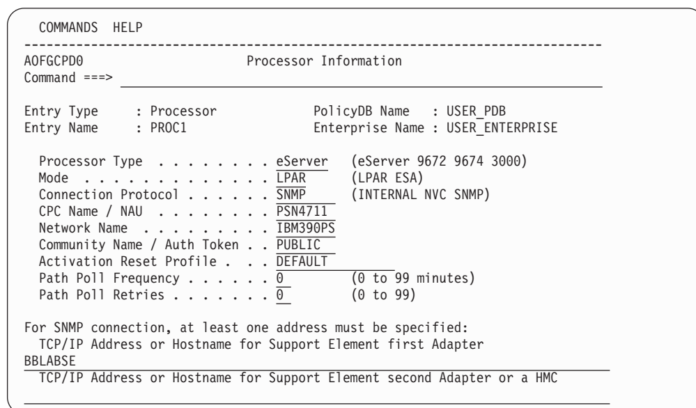
Figure 169. Processor Information Panel
