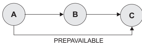
Figure 124. Using STARTUP Policy
