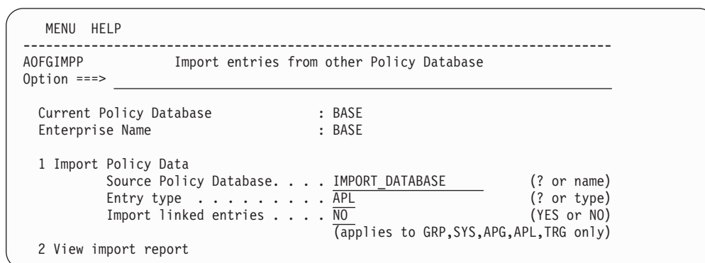
Figure 261. Policy Data Base Import Panel
