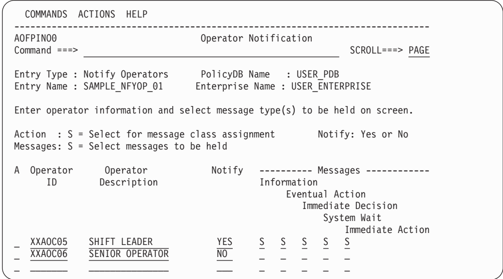
Figure 223. Operator Notification Panel
