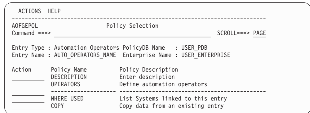
Figure 219. Policy Selection Panel for Automation Operators
