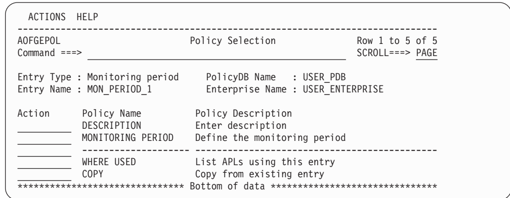
Figure 202. Policy Selection Panel for CICS Link Monitor Periods
