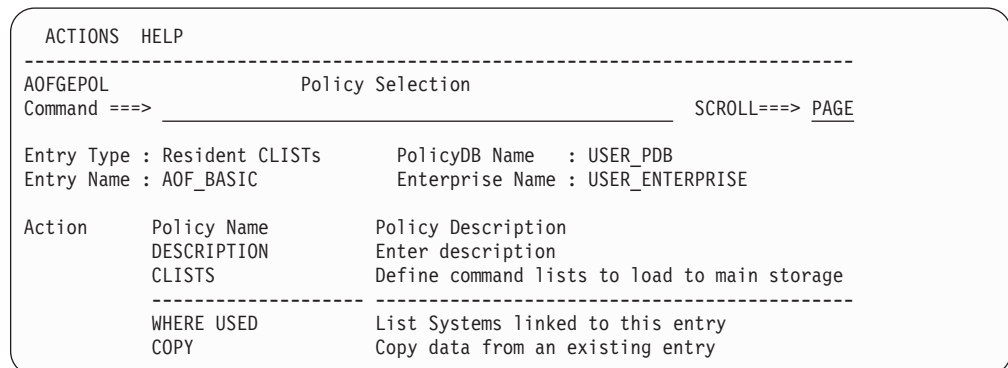
Figure 236. Policy Selection Panel for Resident CLISTs
