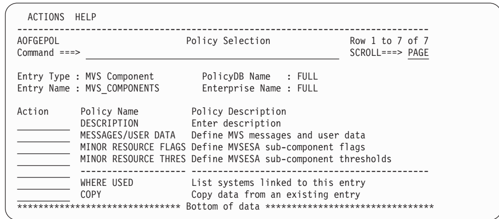
Figure 211. Policy Selection Panel for MVS Components
