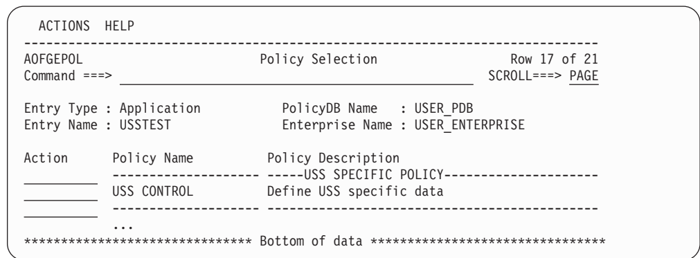
Figure 155. Policy Selection Panel for USS Subsystems
