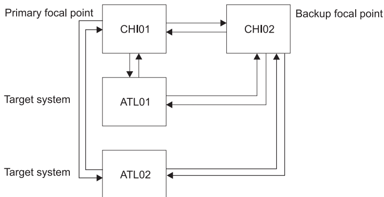
Figure 275. Focal Point Forwarding Definitions for Systems
