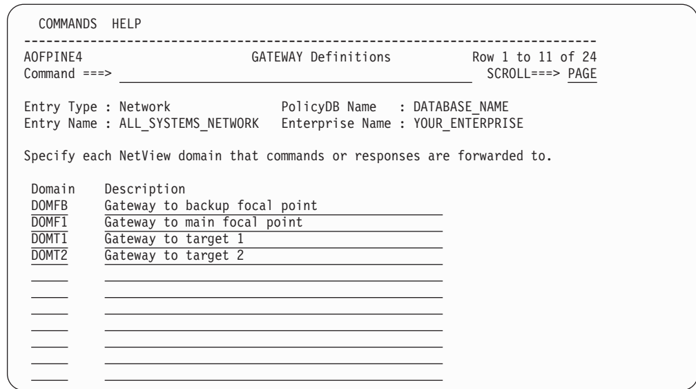
Figure 228. GATEWAY Definitions Panel
