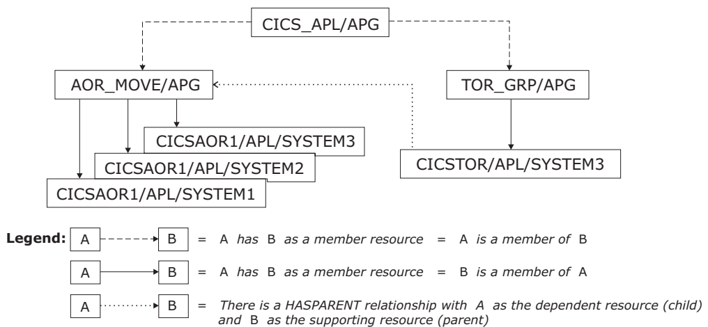
Figure 48. Generated Resources in the Solution
