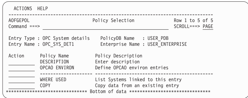
Figure 192. Policy Selection Panel for OPC System Detail
