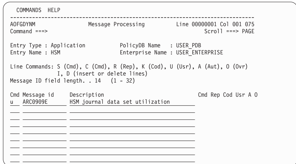
Figure 54. Message Processing Panel
