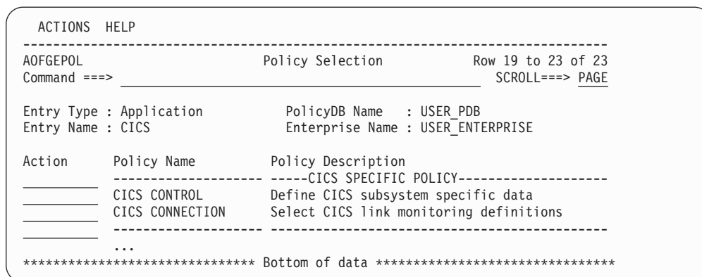
Figure 145. Policy Selection Panel for CICS Subsystems
