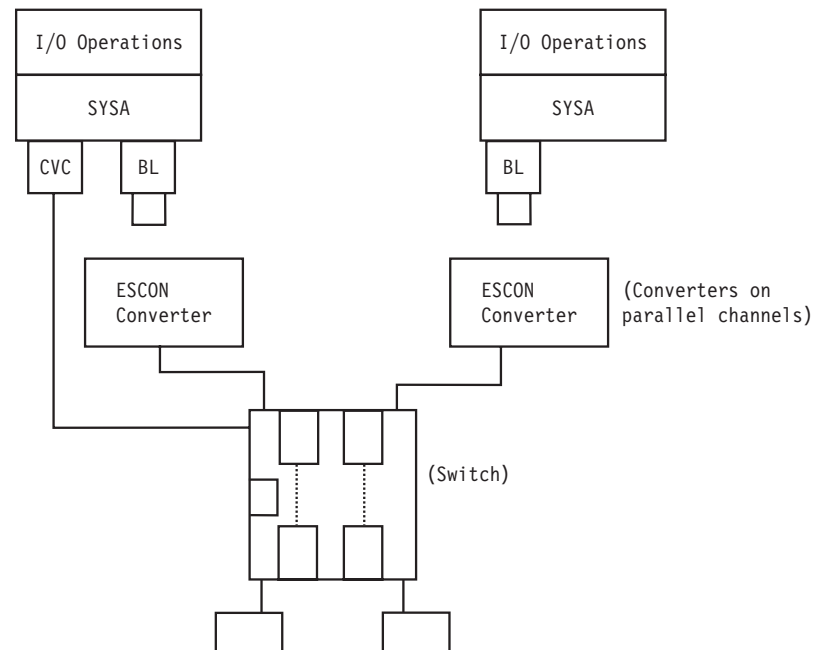
Figure 172. Parallel Channel in Block Mode - Sample.
