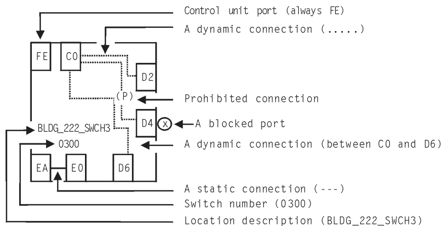
Figure 160. Sample of an ESCON Director Diagram.
