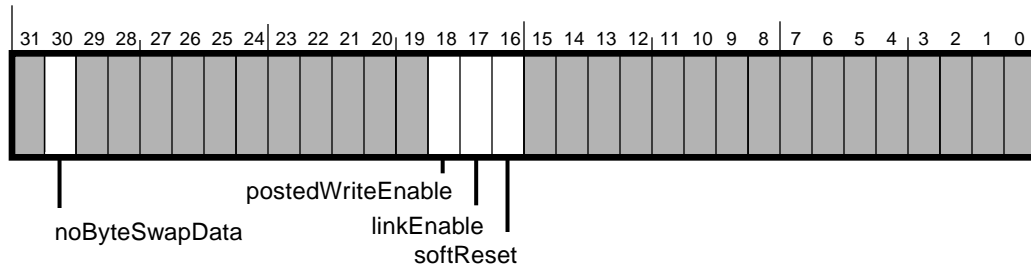
Figure 5-14 — HCControl register
