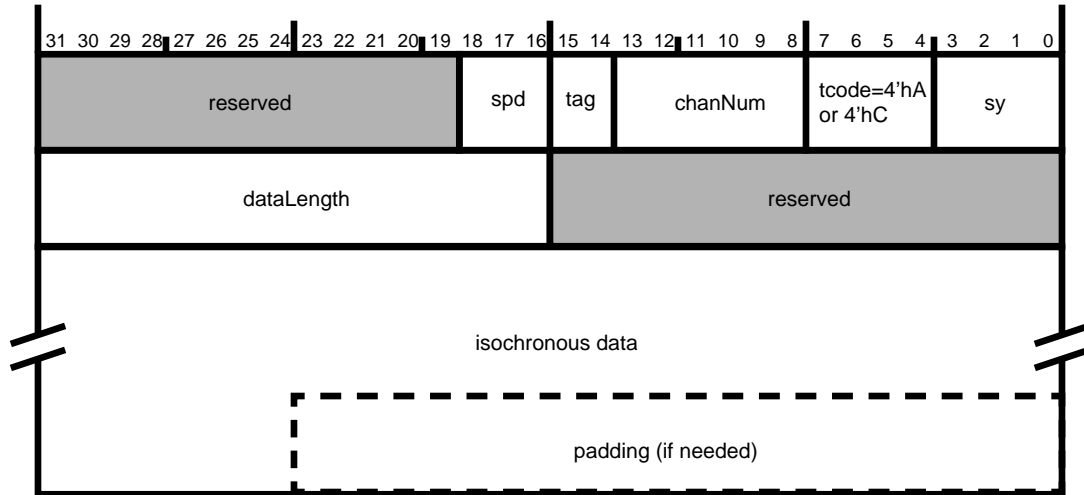
Figure 9-10 — Isochronous transmit format with header/cycleNumber
