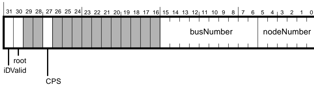
Figure 5-16 — Node ID register
