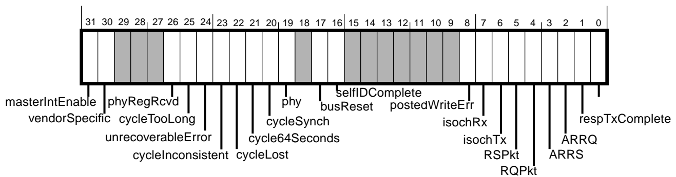
Figure 6-2 — IntMask register
