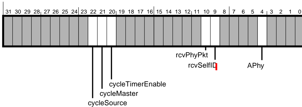
Figure 5-15 — LinkControl register
