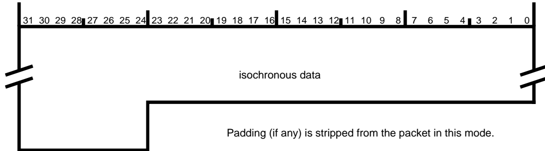
Figure 10-12 — Receive isochronous format in packet-per-buffer mode without header/trailer
