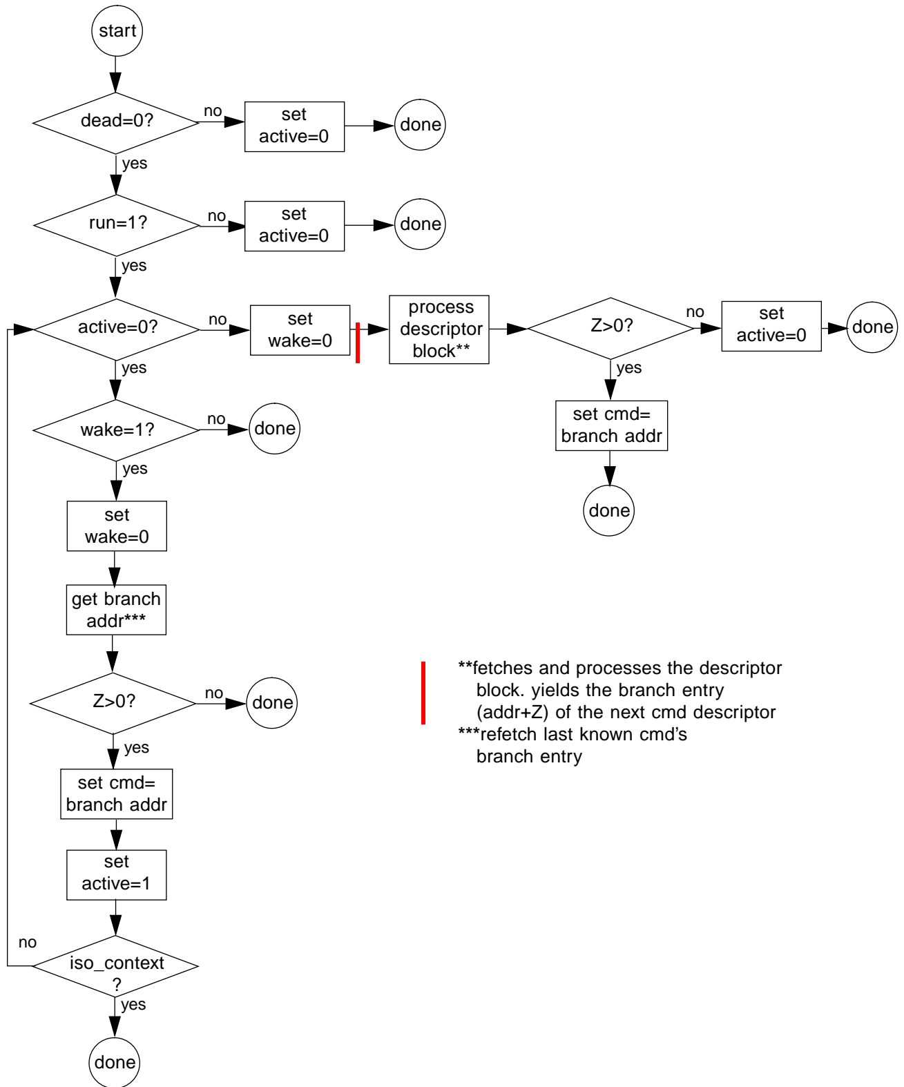
Figure 3-3 — Flow Chart for processing a descriptor
