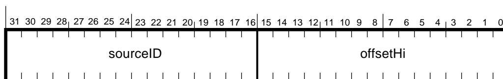
Figure 12-1 — PostedWriteAddressHi register
