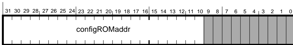
Figure 5-12 — Configuration ROM mapping register
