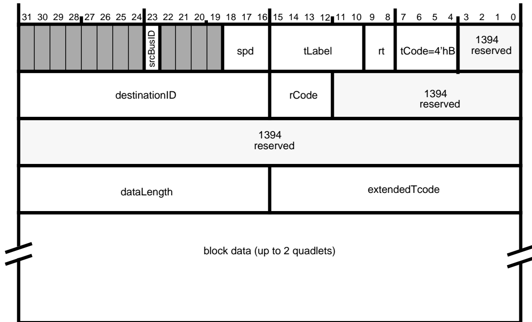
Figure 7-17 — Lock response transmit format
