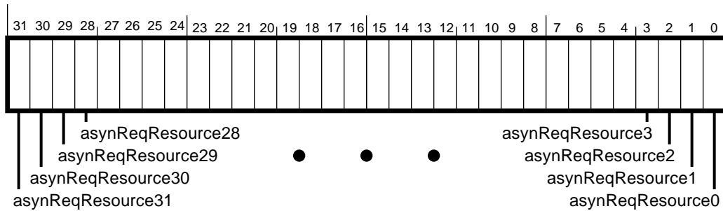
Figure 5-20 — AsynchronousRequestFilterLo (set and clear) register
