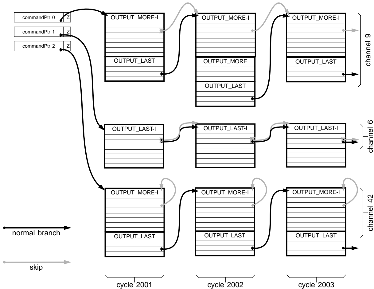
Figure 9-8 — ITDMA summary
