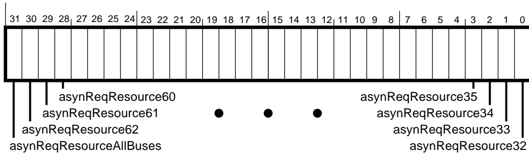
Figure 5-19 — AsynchronousRequestFilterHi (set and clear) register
