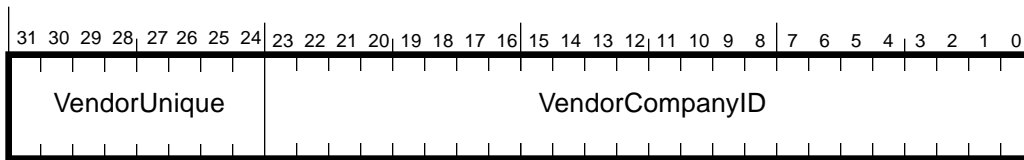
Figure 5-13 — VendorID register
