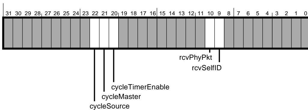
Figure 5-15 — LinkControl register
