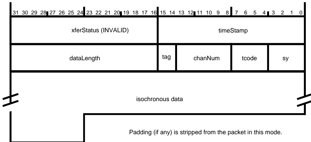
Figure 10-11 — Receive isochronous format in packet-per-buffer mode with header/trailer
