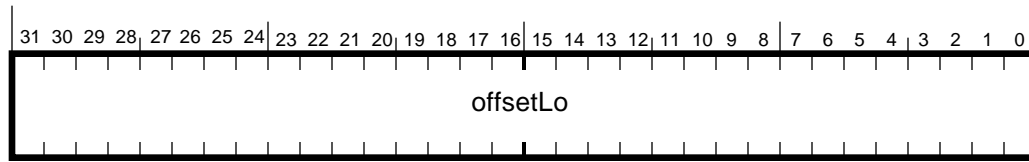
Figure 12-2 — PostedWriteAddressLo register
