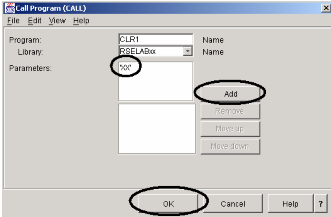
Figure 61: Prompt window
