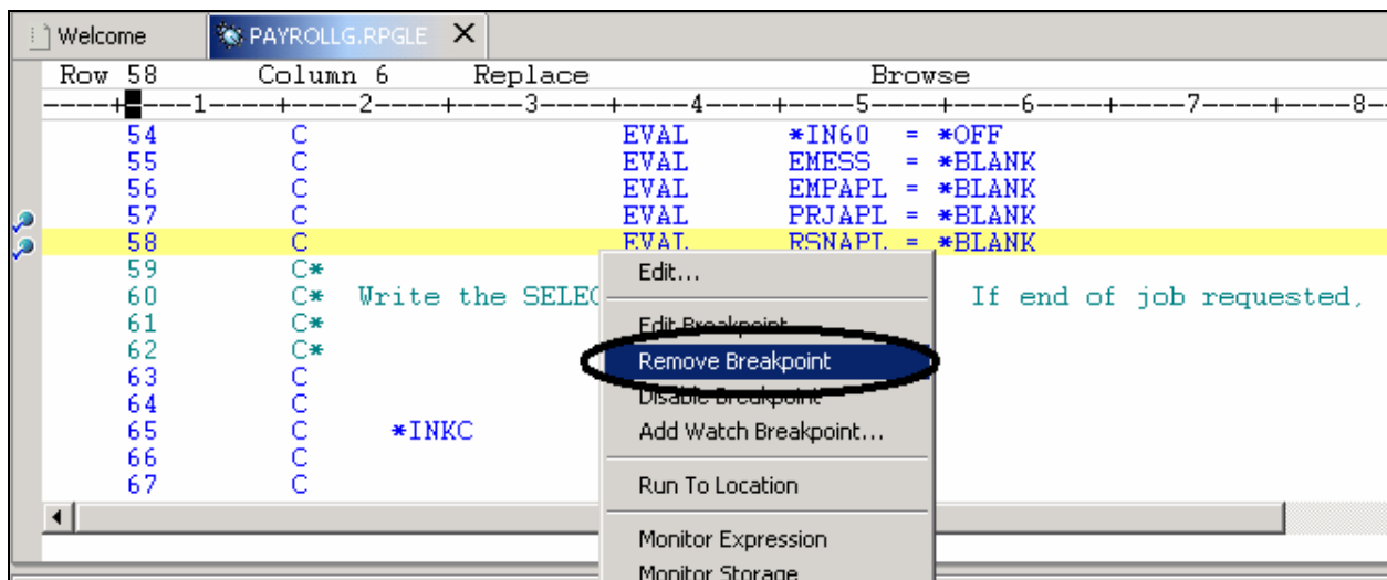
Figure 76: Remove breakpoint
