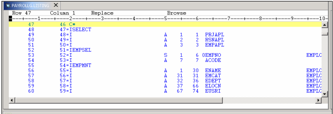
Figure 73: Expanded Input specs for externally described files
