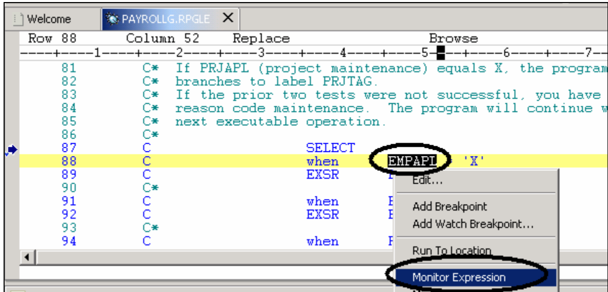
Figure 77: Add variable to monitor
