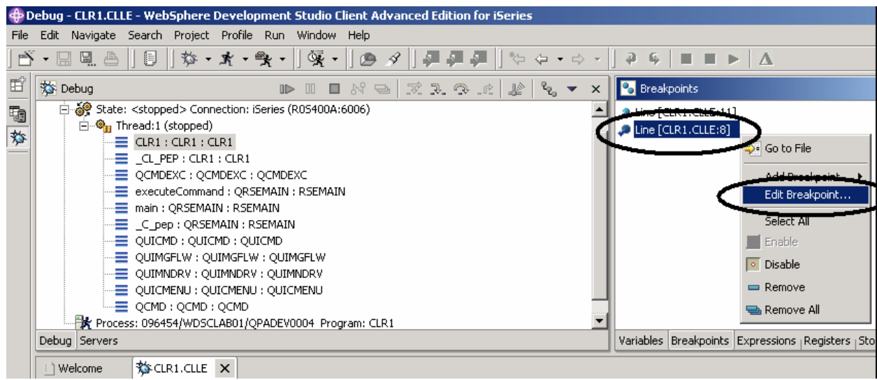
Figure 66: Edit breakpoint in Breakpoint view
