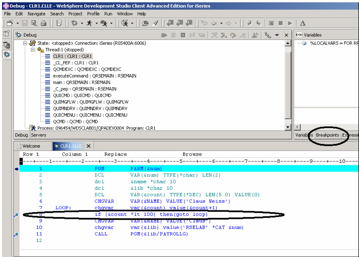
Figure 65: Adding a break point and selecting the breakpoint view
