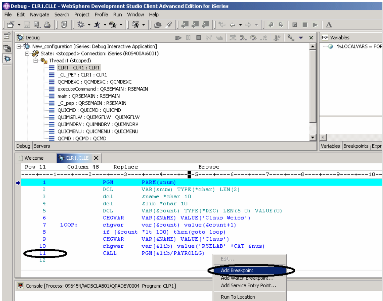
Figure 64: Debug perspective, adding breakpoint
