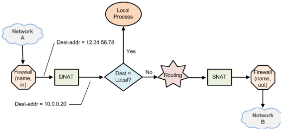
FIGURE 12 Brocade vRouter–destined DNAT routing decisions
