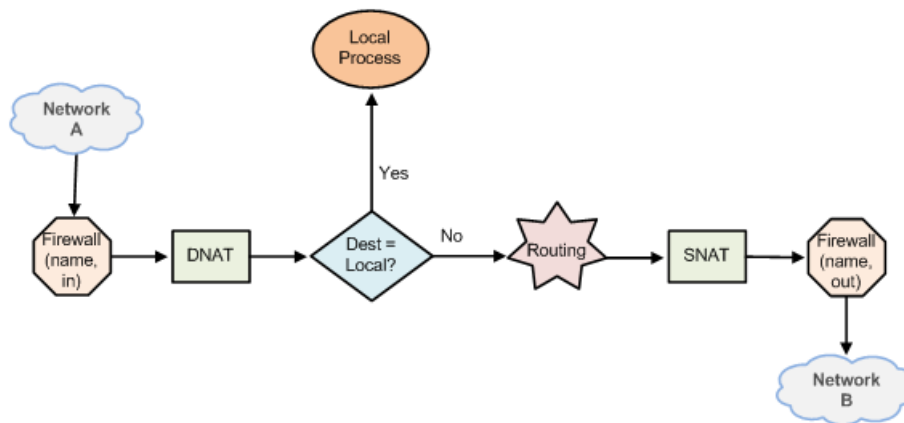
FIGURE 10 Traffic flow through the Brocade vRouter
