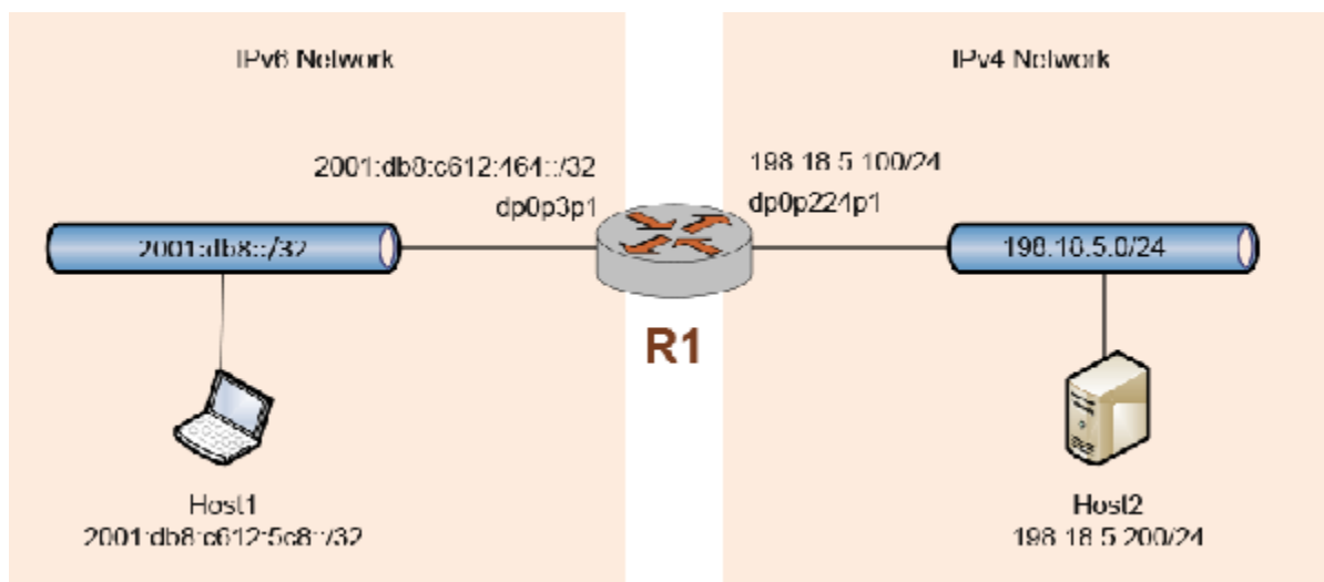
FIGURE 27 NAT 6-4 configuration example
