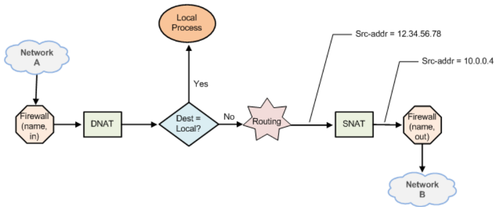
FIGURE 15 Pass-through SNAT firewall decisions
