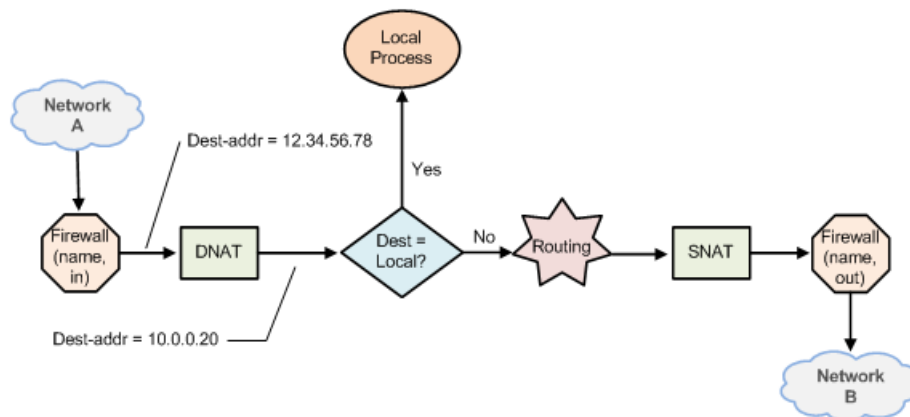
FIGURE 14 Brocade vRouter–destined DNAT firewall decisions
