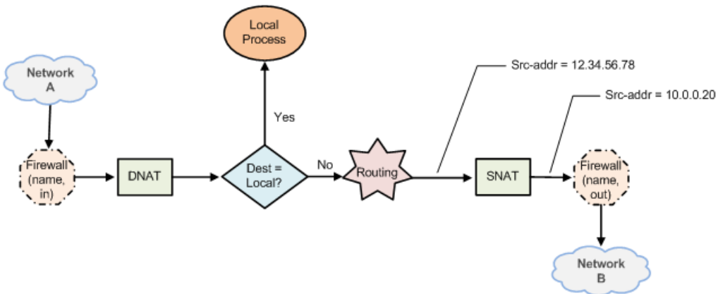
FIGURE 16 Brocade vRouter-originated SNAT firewall decisions
