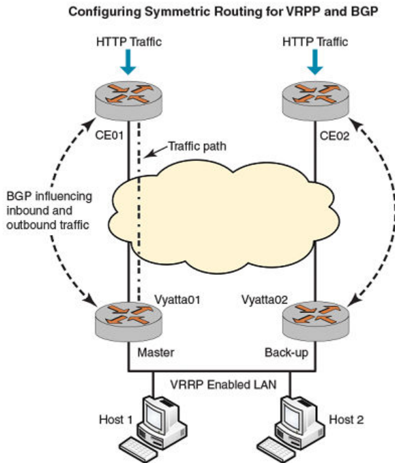
FIGURE 3 Configuring symmetric routing for VRRP and BGP
