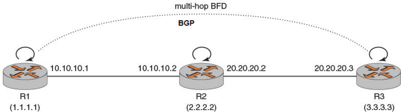
FIGURE 6 Configuring BFD for BGP multiple hop by using IPv4 addressing
