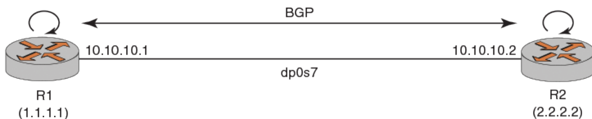
FIGURE 5 Configuring BFD for BGP single hop by using IPv4 addressing
