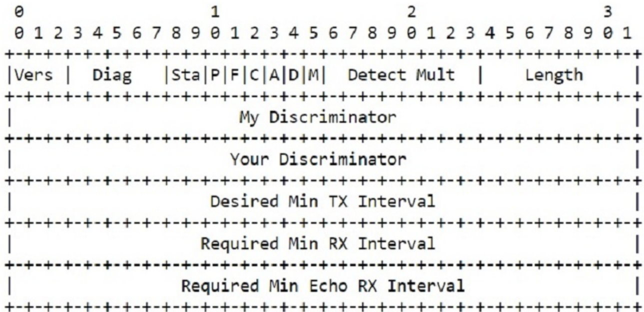
FIGURE 2 Format of a BFD control packet
